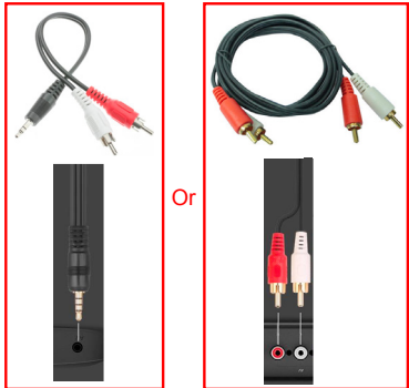
AUX Input depends on the type of jack installed in your car from the factory
