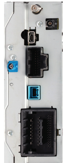
Back of Car Radio
