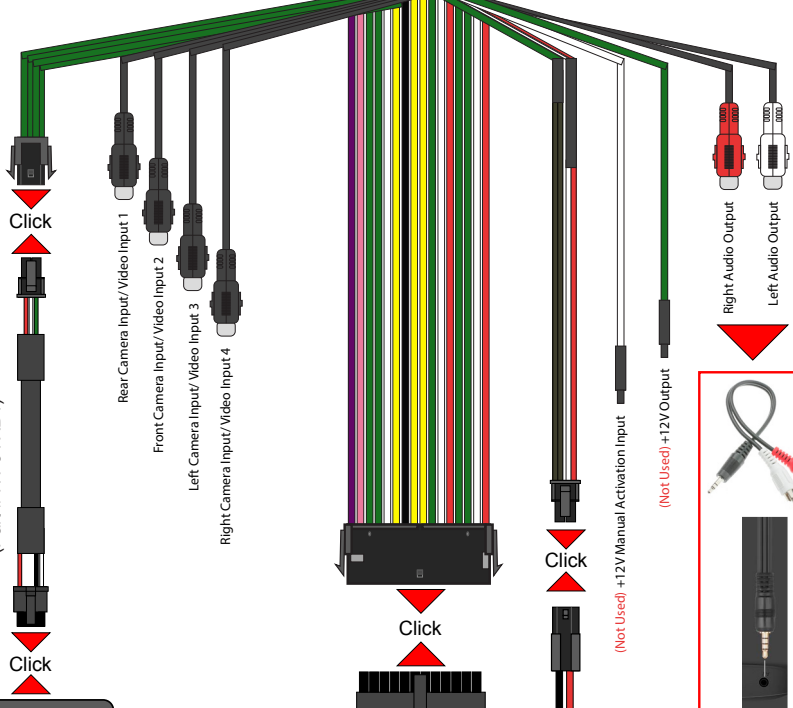
NavTool Interface Harness (Part # NT-WHNT6)
