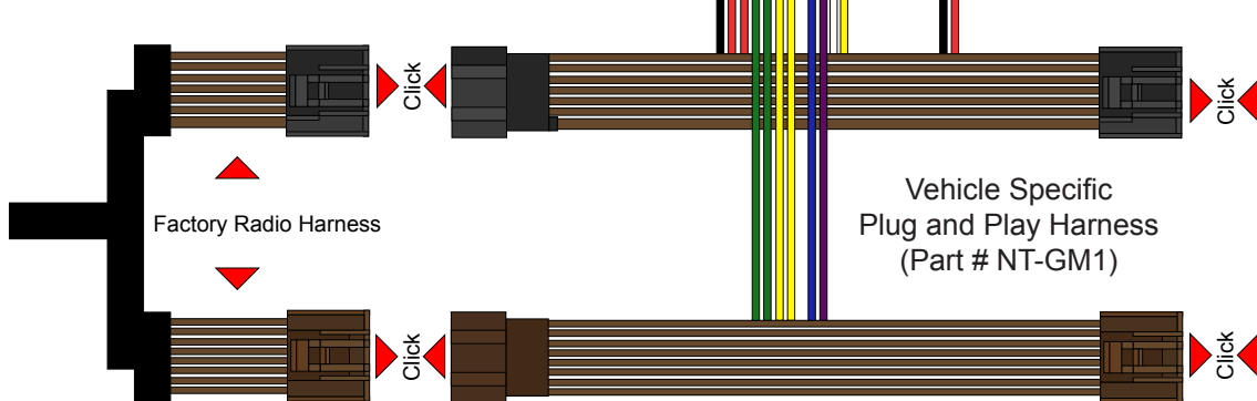
AUX Input depends on the type of jack installed in your car from the factory
